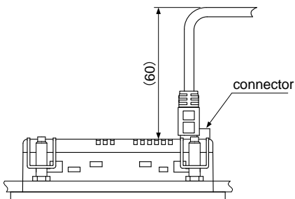
Installation dimensions
